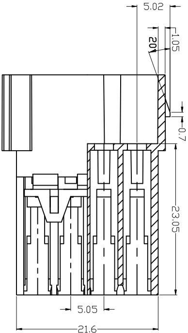
SECTION B-B
