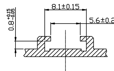
PART. SECT A-A
