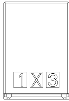
KF7025-06W-2.5AWG (6POS:X-KEY)
