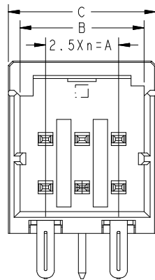
KF7025-06W-2.5AWG (6POS:X-KEY)
