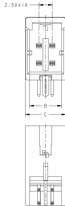
KF7025-04W-2.5AWG (4POS: X-KEY)
