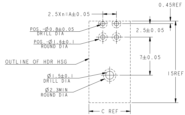
KF7025-04W-2.5AWG (4POS: X-KEY)
