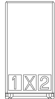
KF7025-04W-2.5AWG (4POS: X-KEY)
