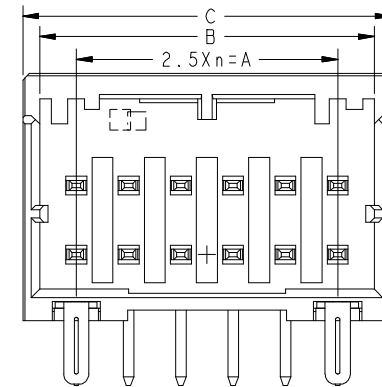
KF7025-12W-2.5AWG (12POS:X-KEY)
