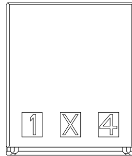
KF7025-08W-2.5AWG (8POS:X-KEY)
