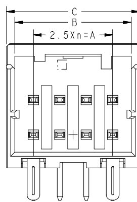
KF7025-08W-2.5AWG (8POS:X-KEY)
