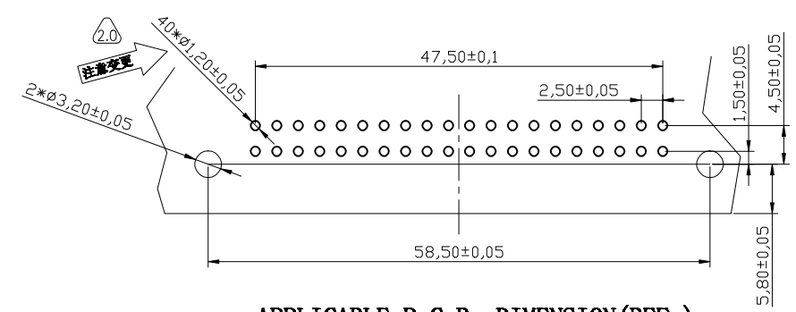
APPLICABLE P. C. B. DIMENSION (REF.)
